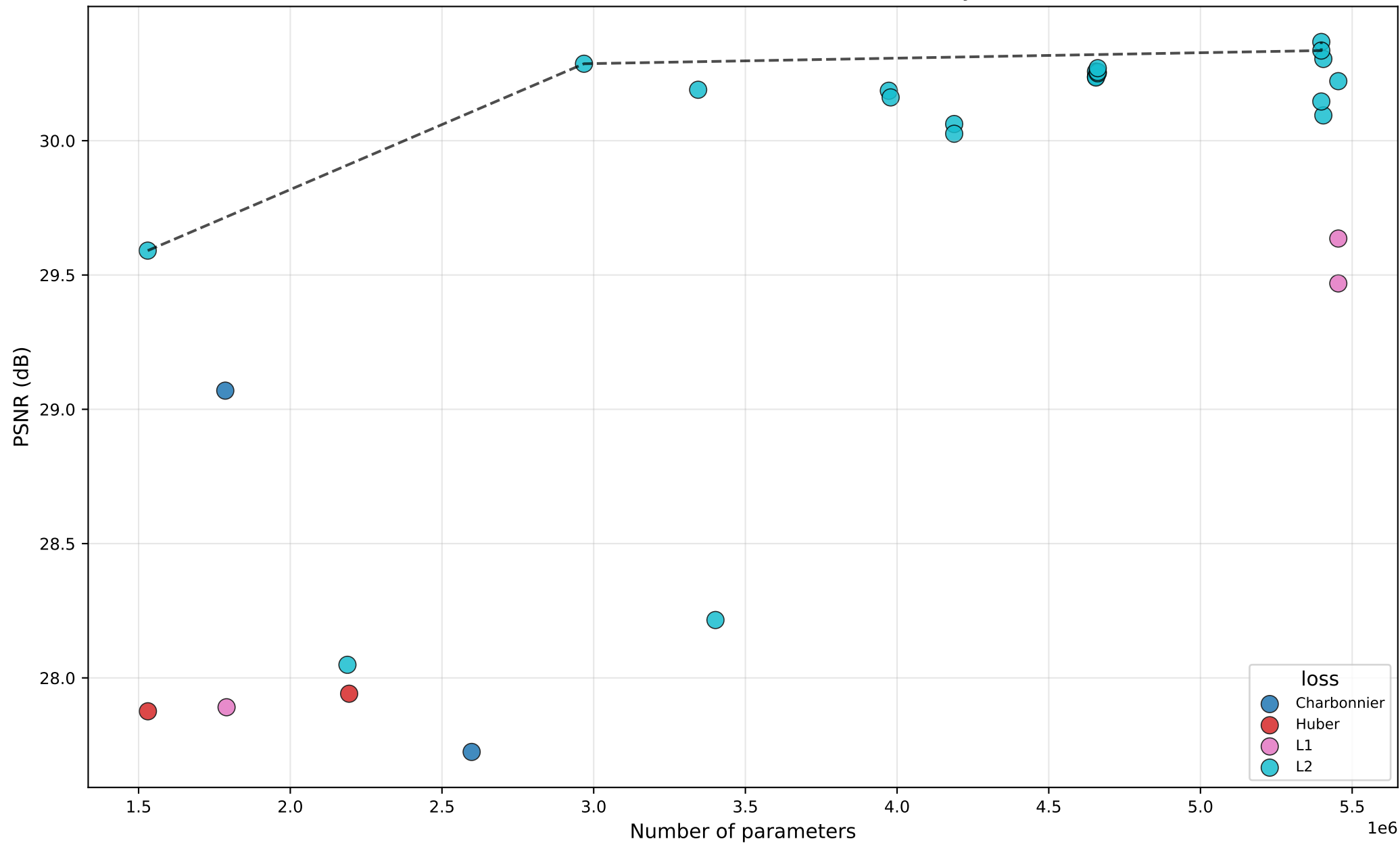
PSNR vs #Params — WaveletAttention — by loss
